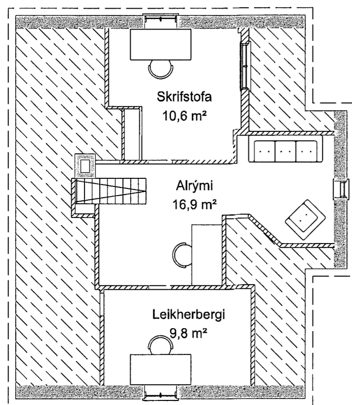
Rishæð; 1:100
