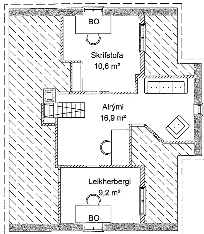
Rishæð; 1:100
